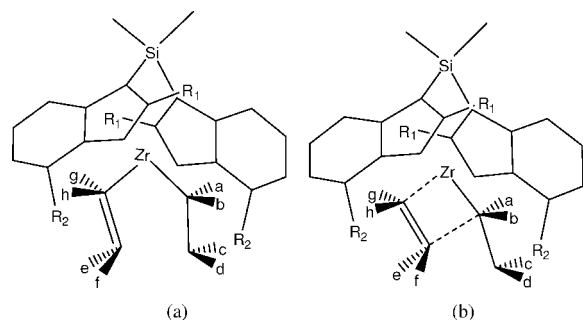
Figure 3. Structures of the α-agostic species (left) and the transition-state for olefin propagation (right).
